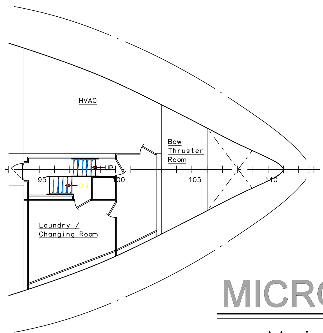
Accommodation Deck
