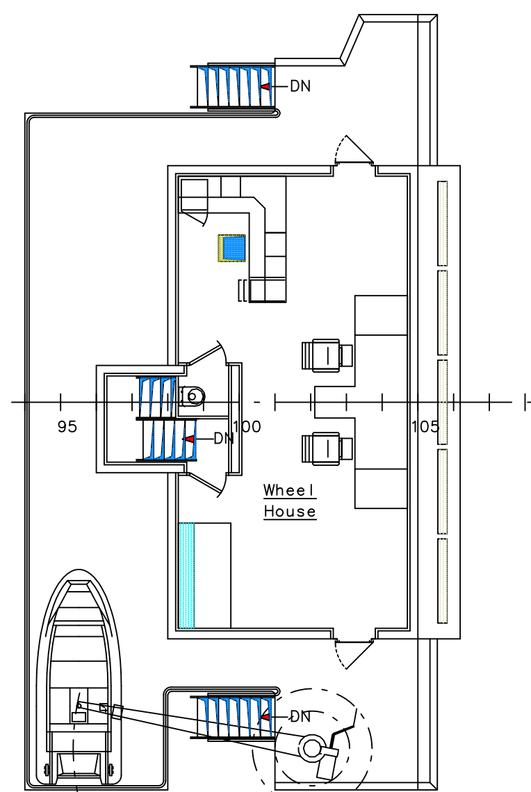
Wheelhouse Deck
